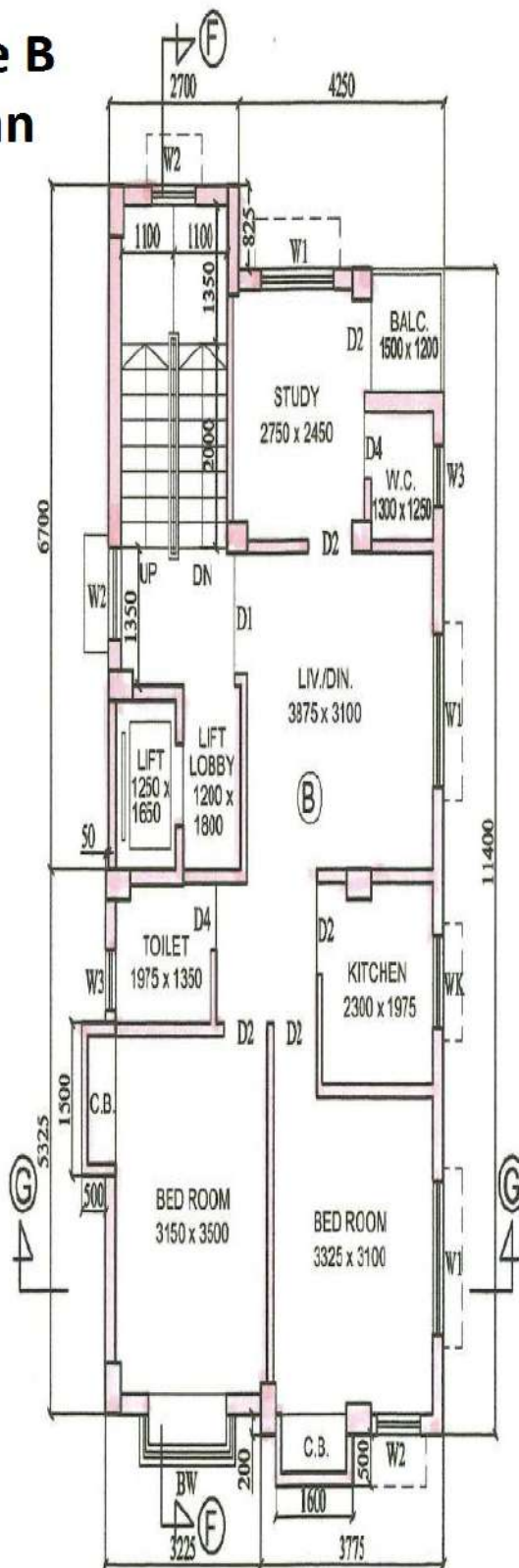
TYPICAL FLOOR PLAN (2ND. TO 4TH. FLOOR SIMILAR)
